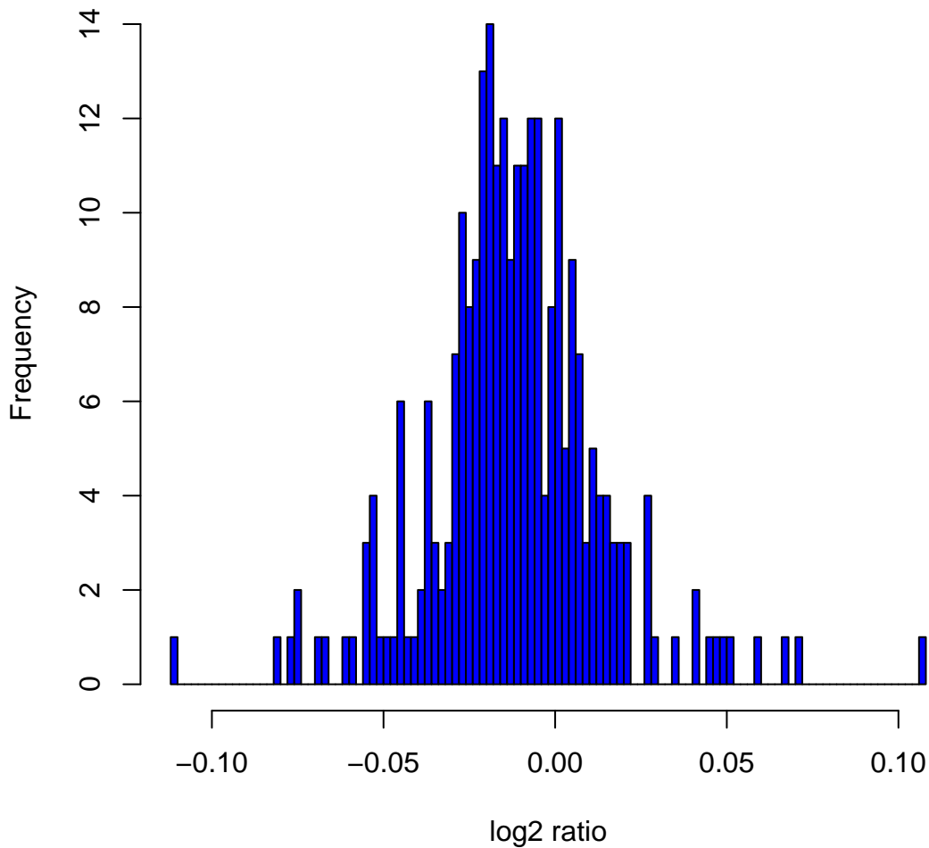
Histogram of log2ratios in 270 HapMap samples at clone Chr1tp-26A11
