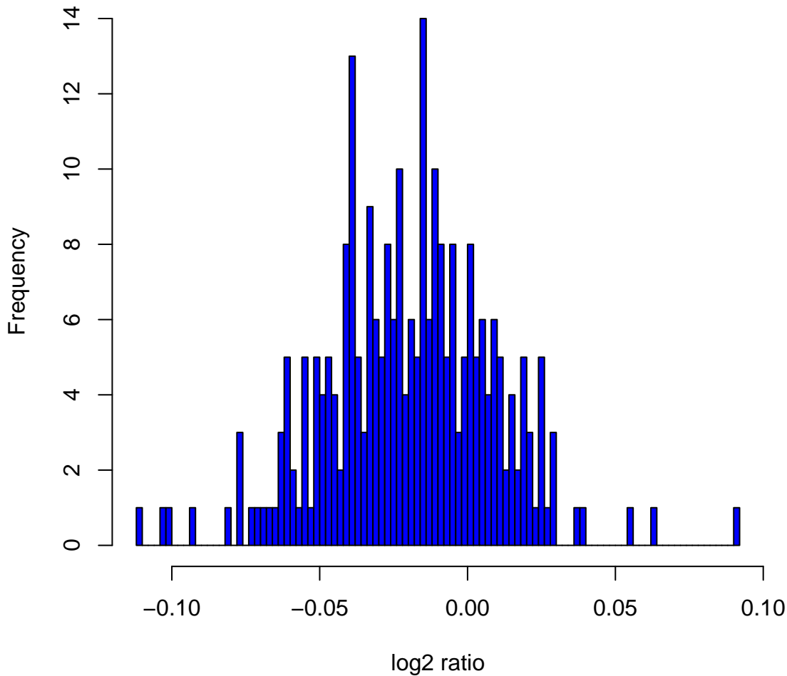
Histogram of log 2 ratios in 270 HapMap samples at clone Chr1tp-26E1
