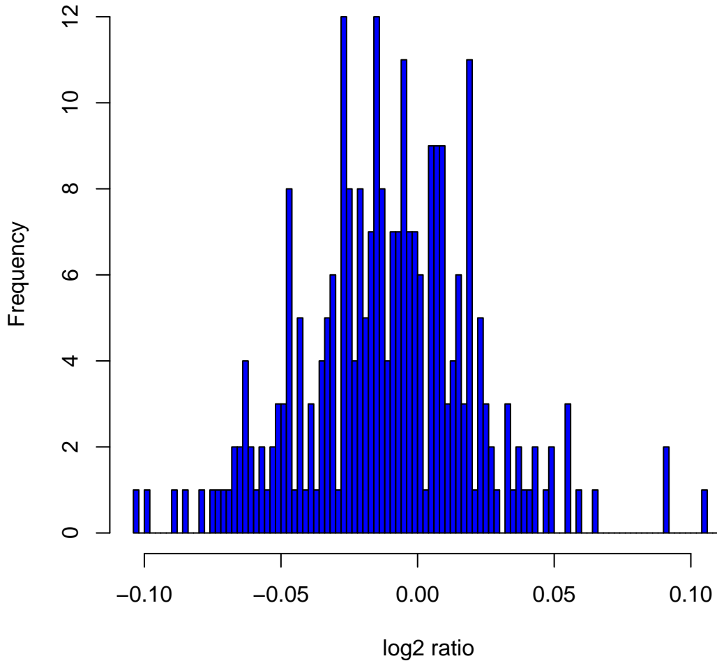
Histogram of \log_2 ratios in 270 HapMap samples at clone Chr1tp-27A2
