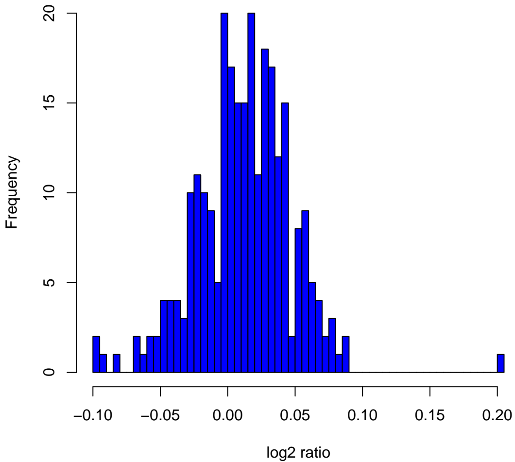
Histogram of log 2 ratios in 270 HapMap samples at clone Chr1tp-27A9
