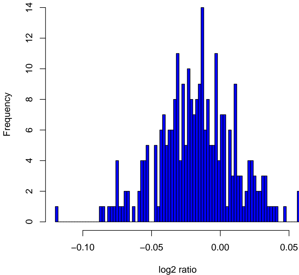
Histogram of log2ratios in 270 HapMap samples at clone Chr1tp-27C12
