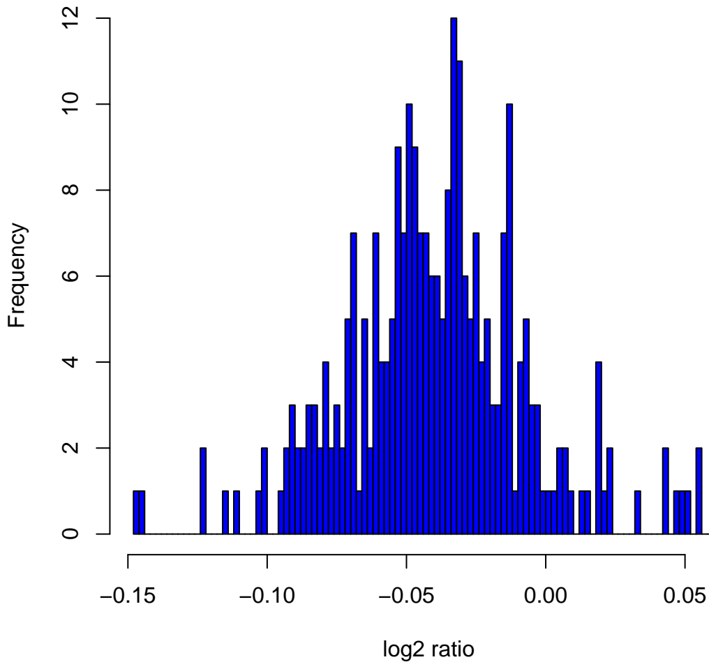
Histogram of log 2 ratios in 270 HapMap samples at clone Chr1tp-27E4
