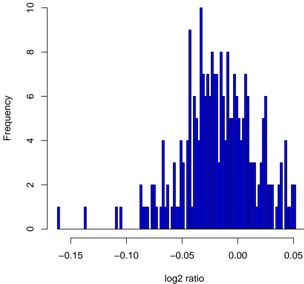
Histogram of log 2 ratios in 270 HapMap samples at clone Chr1tp-27F1
