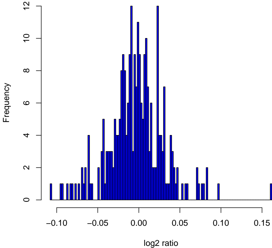
Histogram of log 2 ratios in 270 HapMap samples at clone Chr1tp-28A7
