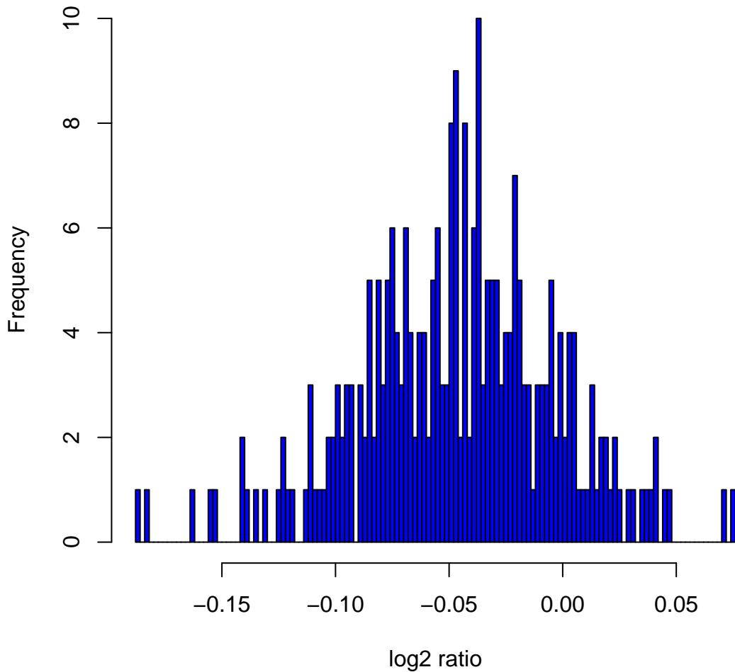
Histogram of log 2 ratios in 270 HapMap samples at clone Chr1tp-29G1
