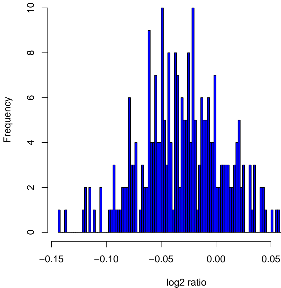
Histogram of \log_2 ratios in 270 HapMap samples at clone Chr1tp-29G2
