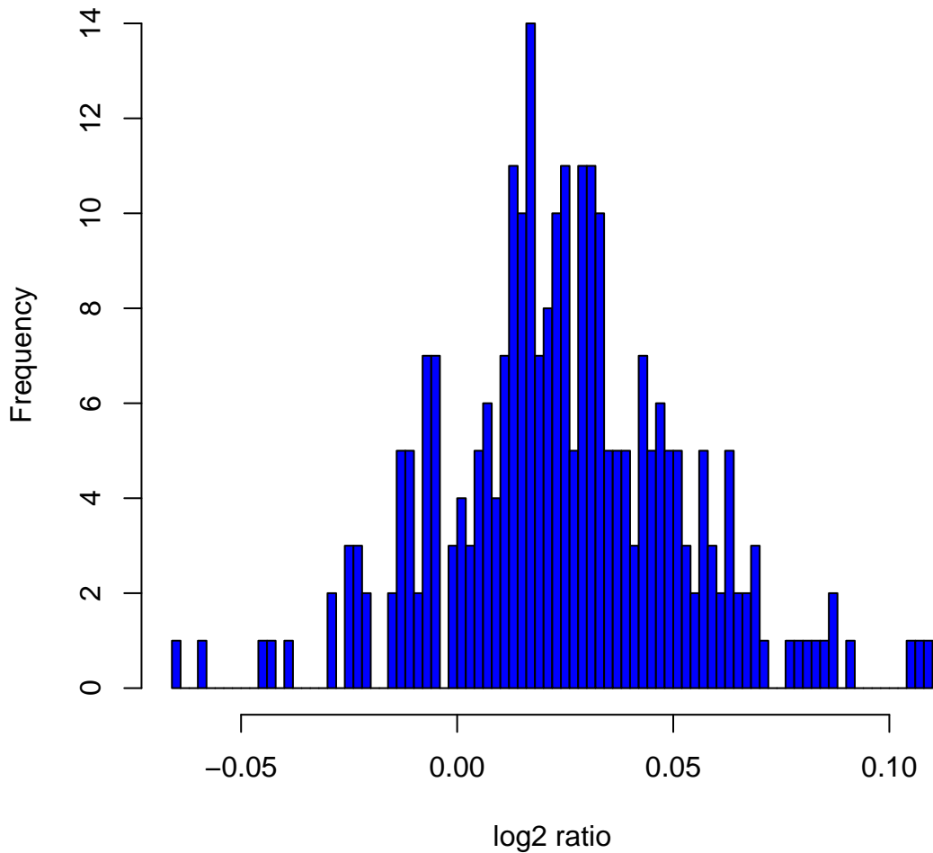
Histogram of log 2 ratios in 270 HapMap samples at clone Chr1tp-29G6
