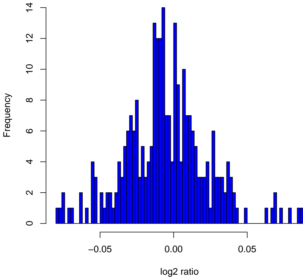
Histogram of log 2 ratios in 270 HapMap samples at clone Chr1tp-29H8
