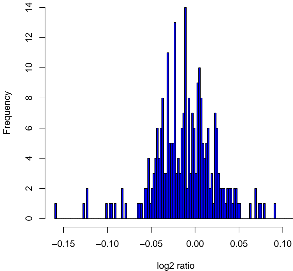
Histogram of \log_2 ratios in 270 HapMap samples at clone Chr1tp-2A5
