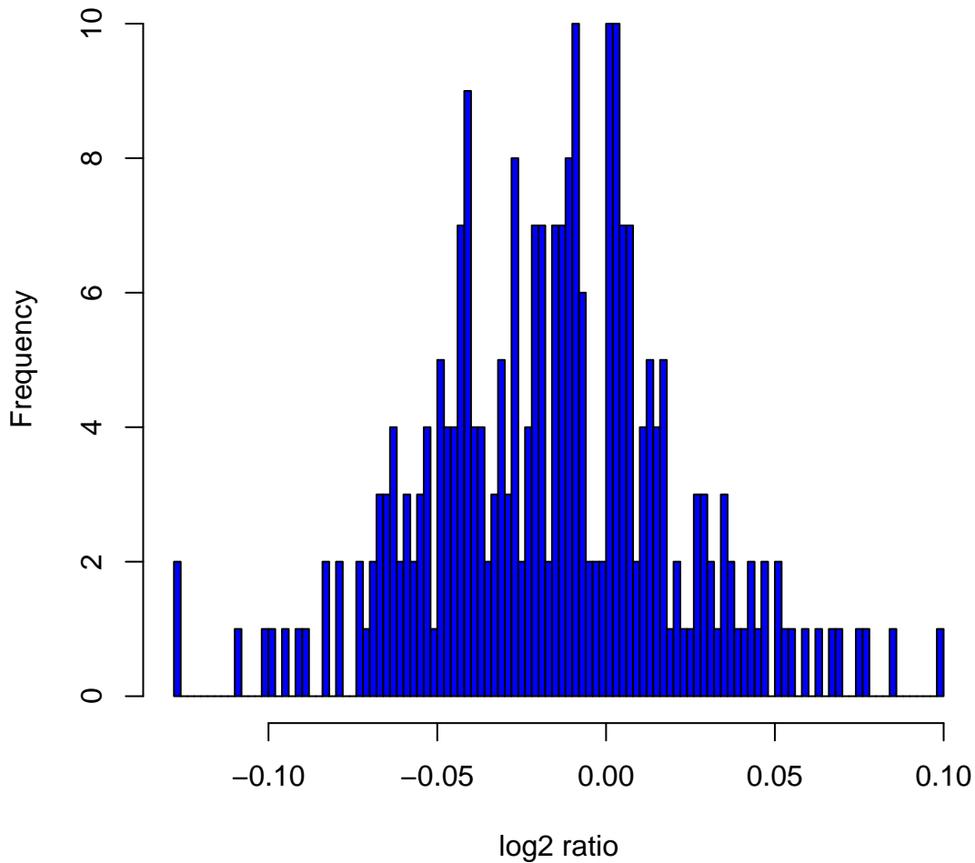
Histogram of log 2 ratios in 270 HapMap samples at clone Chr1tp-2B1
