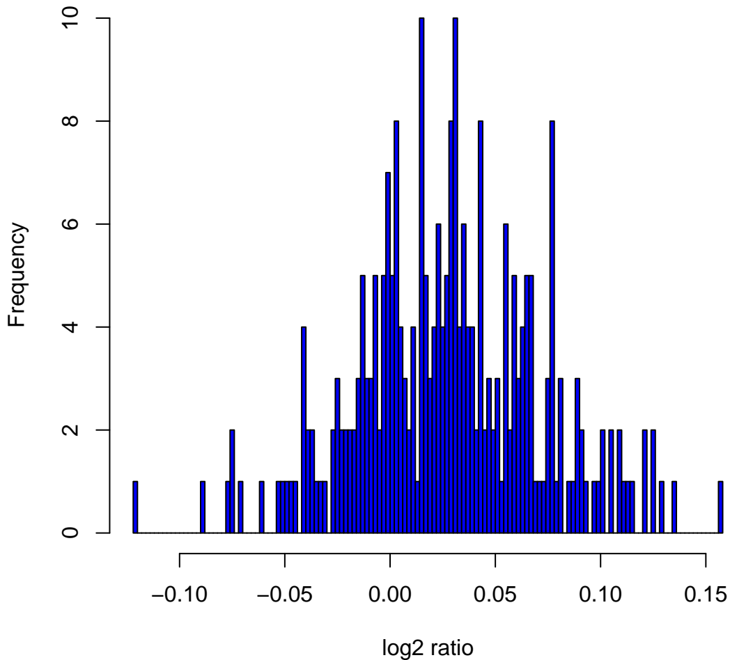
Histogram of log 2 ratios in 270 HapMap samples at clone Chr1tp-2D1
