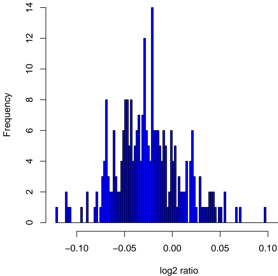
Histogram of log2ratios in 270 HapMap samples at clone Chr1tp-2E2
