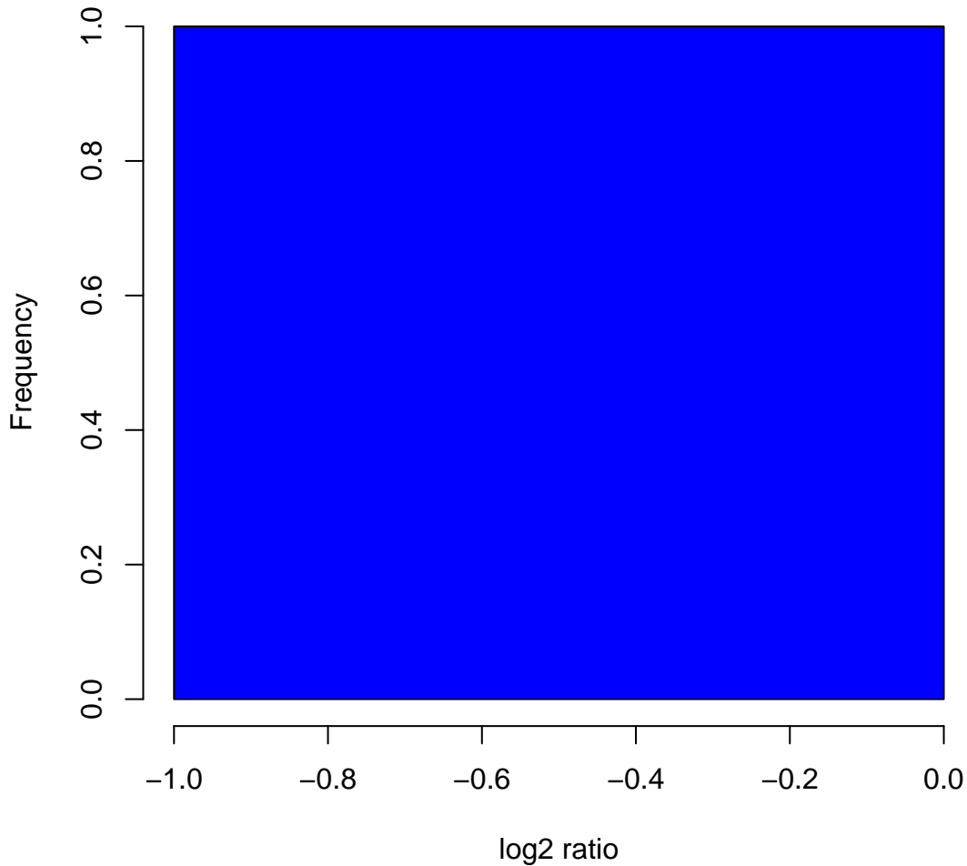
Histogram of log 2 ratios in 270 HapMap samples at clone Chr1tp-2G1
