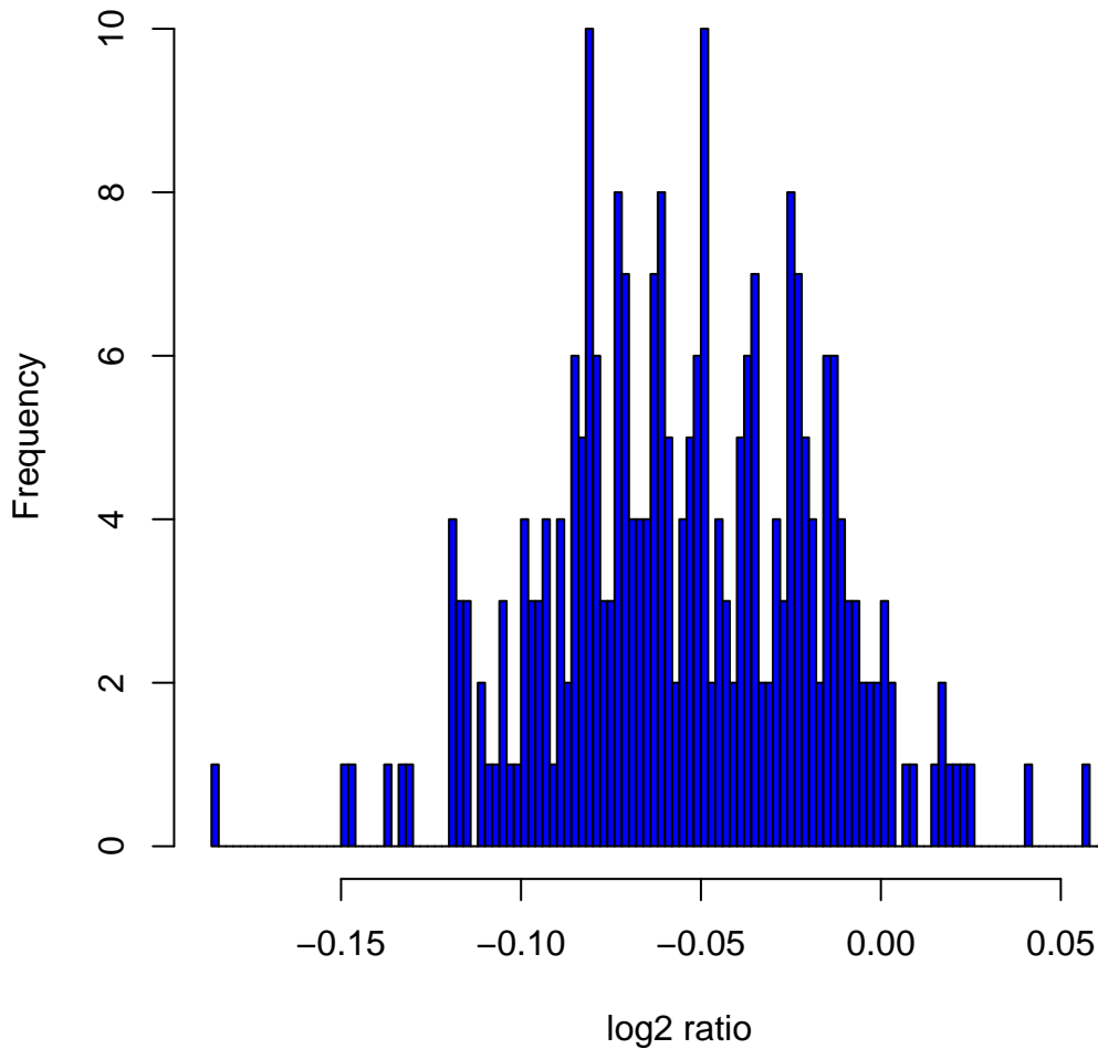
Histogram of \log_2 ratios in 270 HapMap samples at clone Chr1tp-2G2
