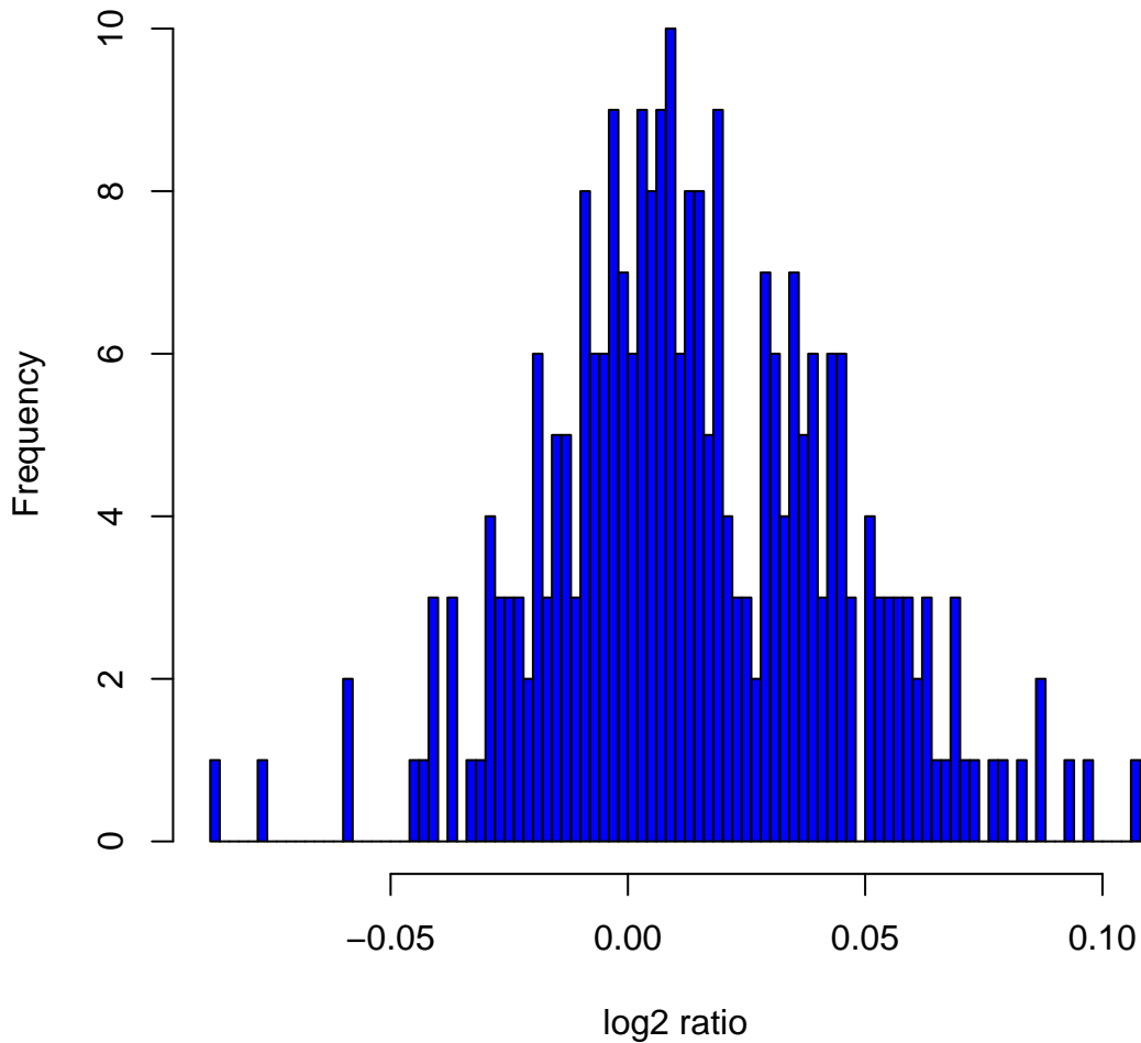
Histogram of log 2 ratios in 270 HapMap samples at clone Chr1tp-30A1
