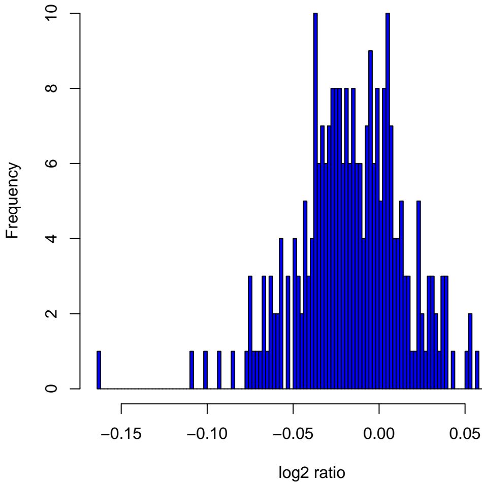
Histogram of log2ratios in 270 HapMap samples at clone Chr1tp-30D12
