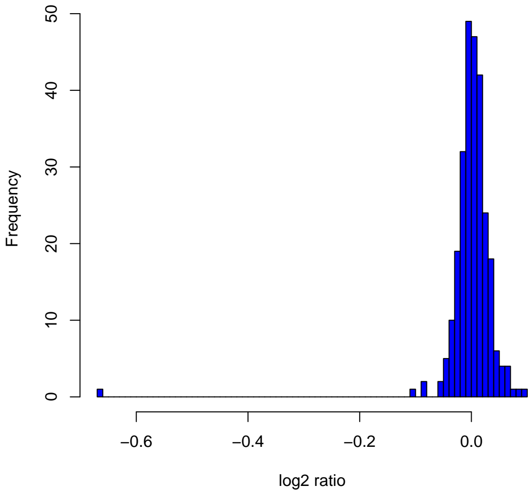
Histogram of log2ratios in 270 HapMap samples at clone Chr1tp-30F10
