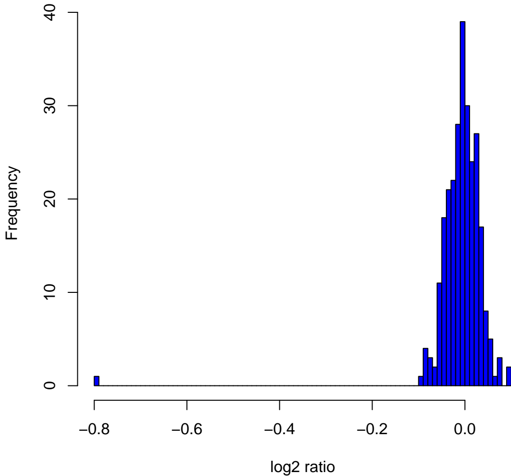
Histogram of log2ratios in 270 HapMap samples at clone Chr1tp-30F5
