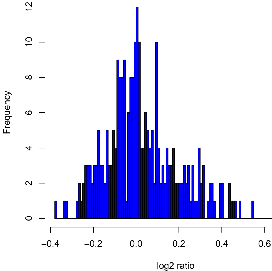
Histogram of log 2 ratios in 270 HapMap samples at clone Chr1tp-30H5
