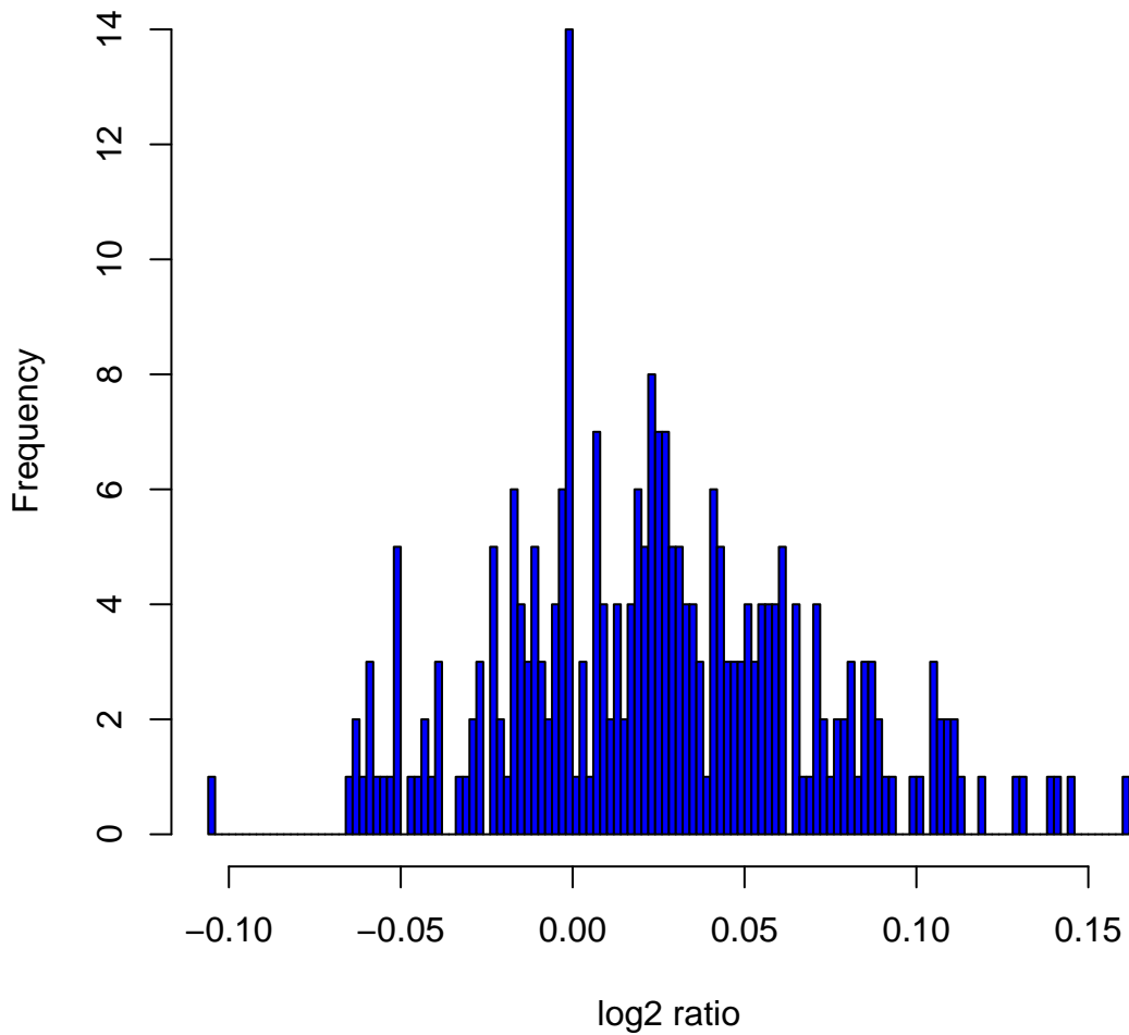
Histogram of log2ratios in 270 HapMap samples at clone Chr1tp-31B3
