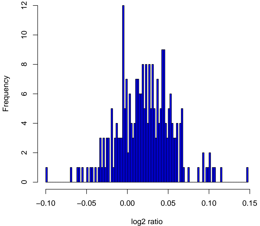
Histogram of log2ratios in 270 HapMap samples at clone Chr1tp-31C11
