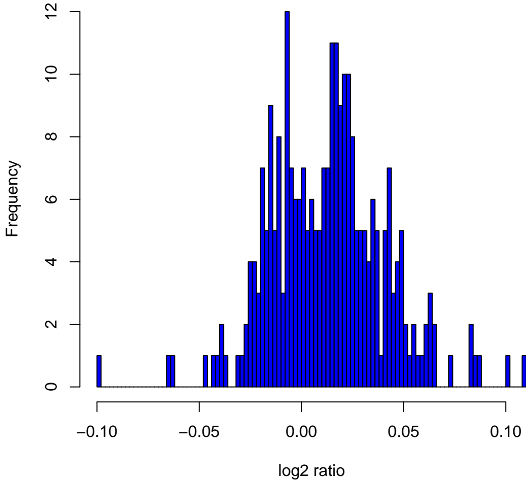
Histogram of log 2 ratios in 270 HapMap samples at clone Chr1tp-31C7
