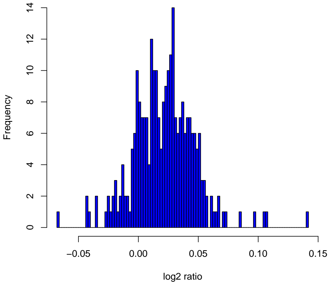
Histogram of log2ratios in 270 HapMap samples at clone Chr1tp-31G11
