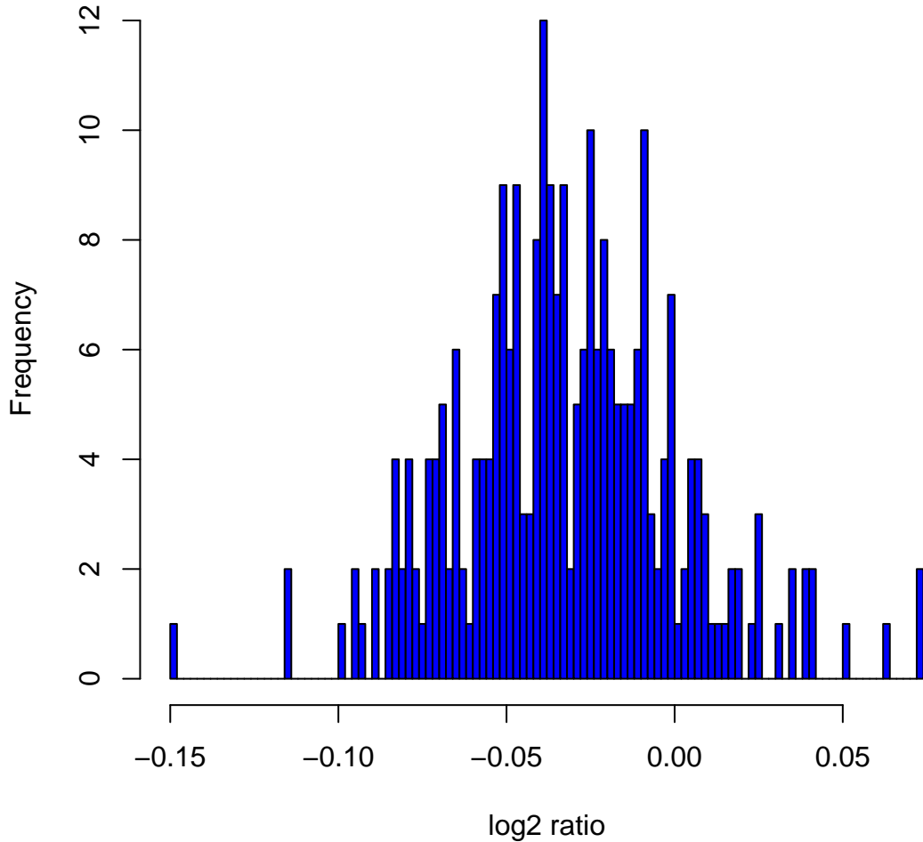
Histogram of log 2 ratios in 270 HapMap samples at clone Chr1tp-31G3
