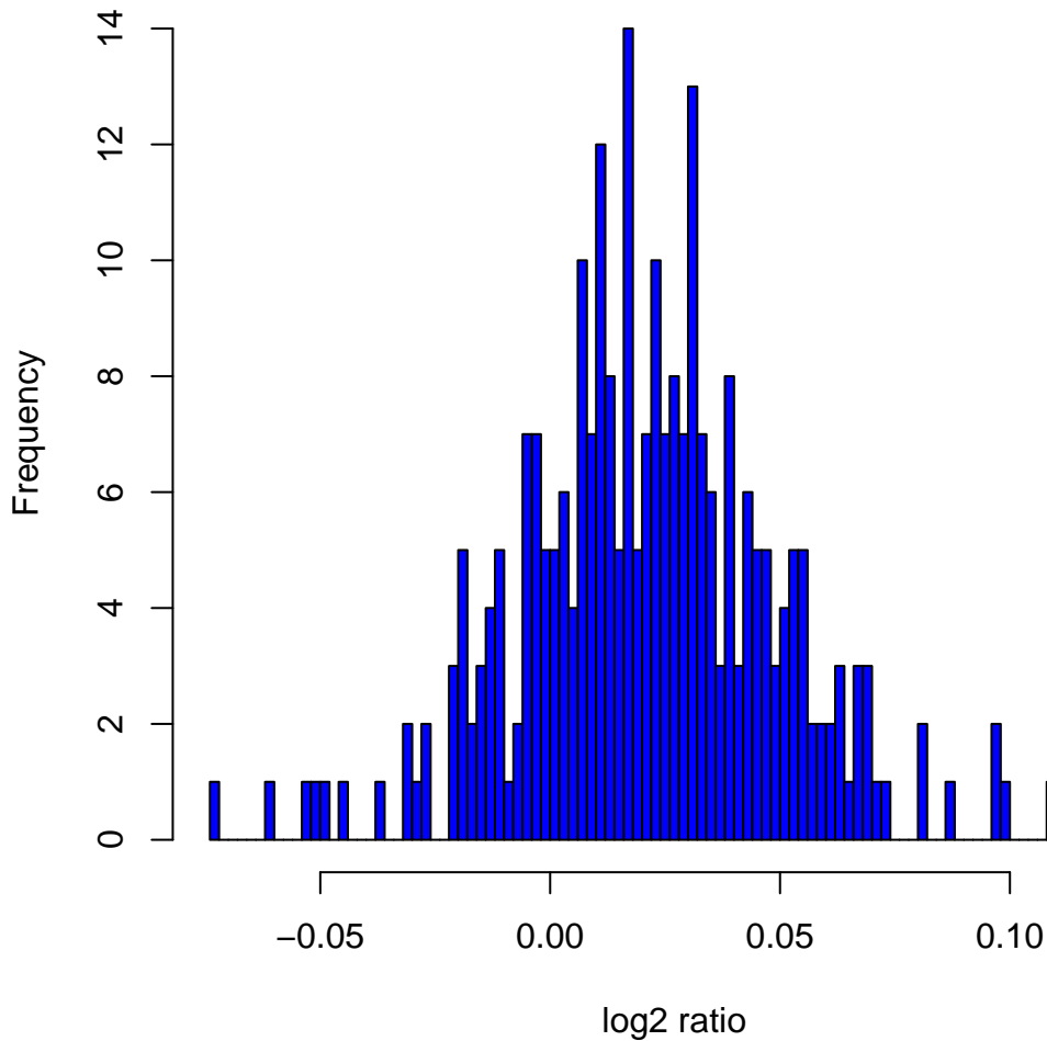
Histogram of log2ratios in 270 HapMap samples at clone Chr1tp-31G9
