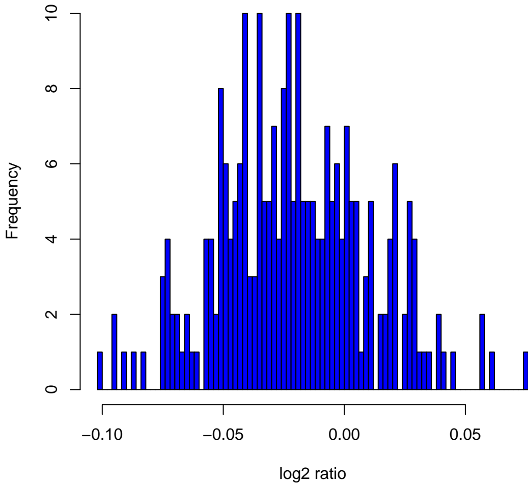
Histogram of log 2 ratios in 270 HapMap samples at clone Chr1tp-32B1
