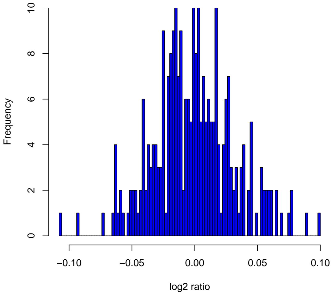
Histogram of \log_2 ratios in 270 HapMap samples at clone Chr1tp-32B6
