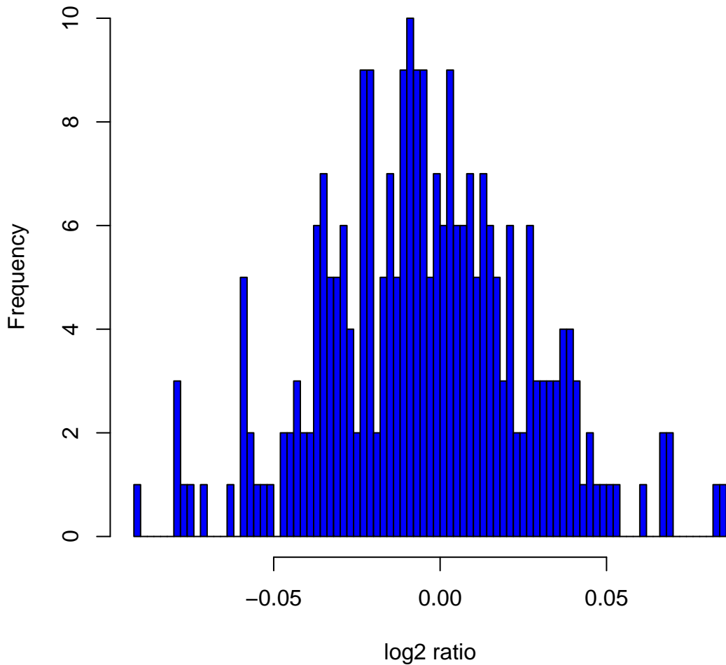
Histogram of log2ratios in 270 HapMap samples at clone Chr1tp-32D10
