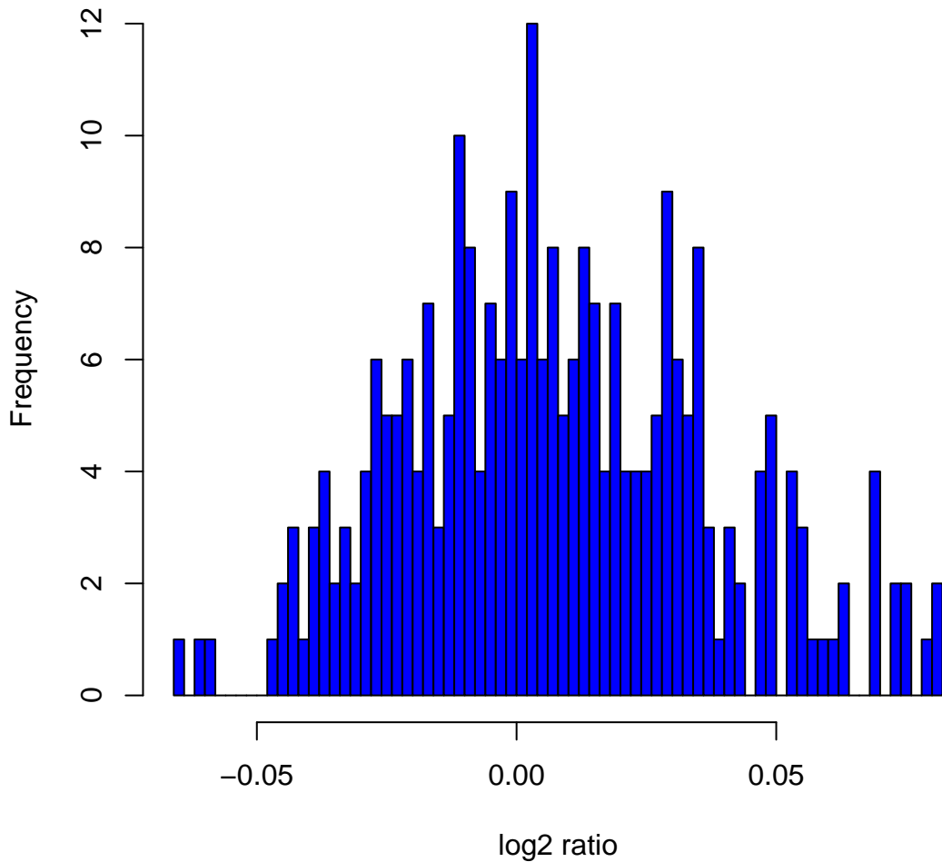
Histogram of log2ratios in 270 HapMap samples at clone Chr1tp-32E11
