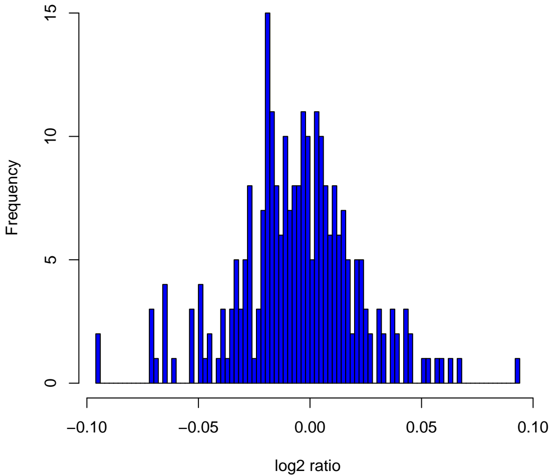
Histogram of log 2 ratios in 270 HapMap samples at clone Chr1tp-32F7
