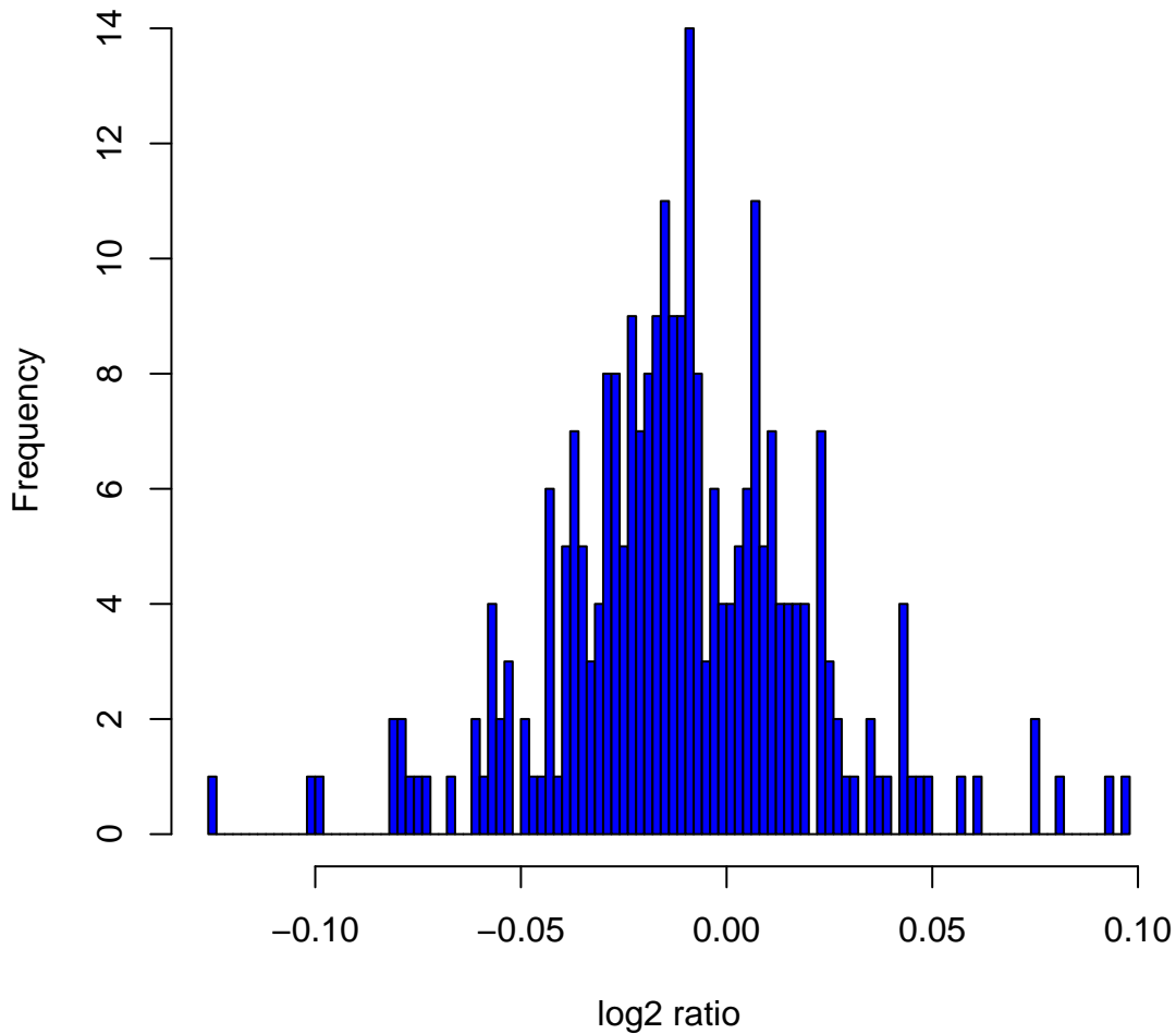
Histogram of log2ratios in 270 HapMap samples at clone Chr1tp-33A10
