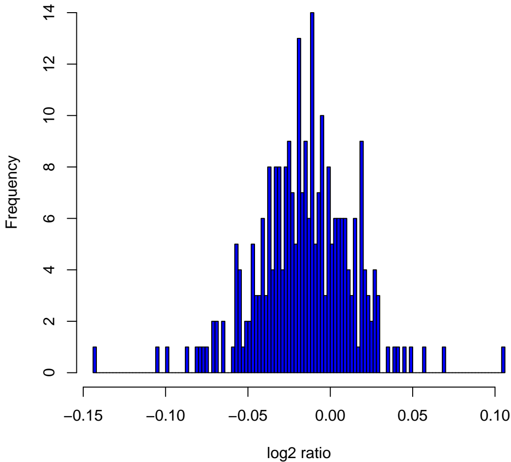
Histogram of log2ratios in 270 HapMap samples at clone Chr1tp-33A12
