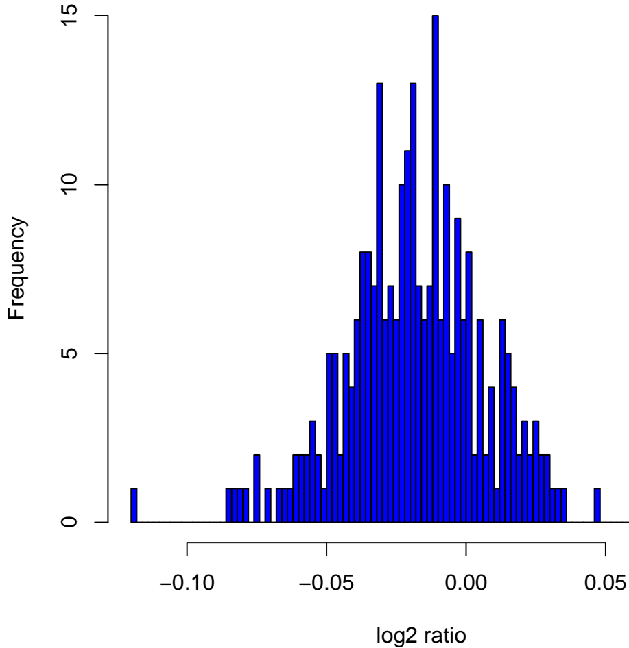
Histogram of log 2 ratios in 270 HapMap samples at clone Chr1tp-33B2
