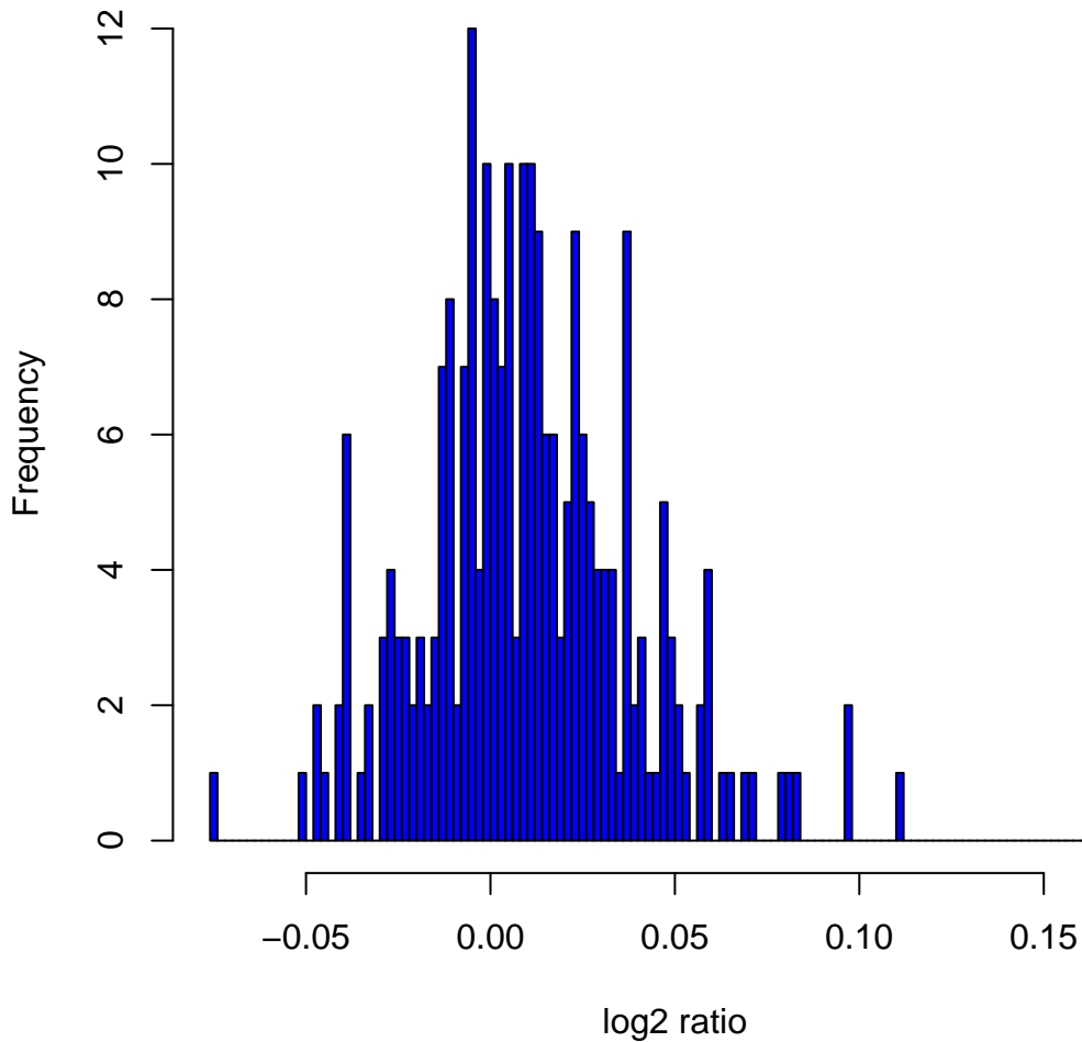
Histogram of \log_2 ratios in 270 HapMap samples at clone Chr1tp-34C1
