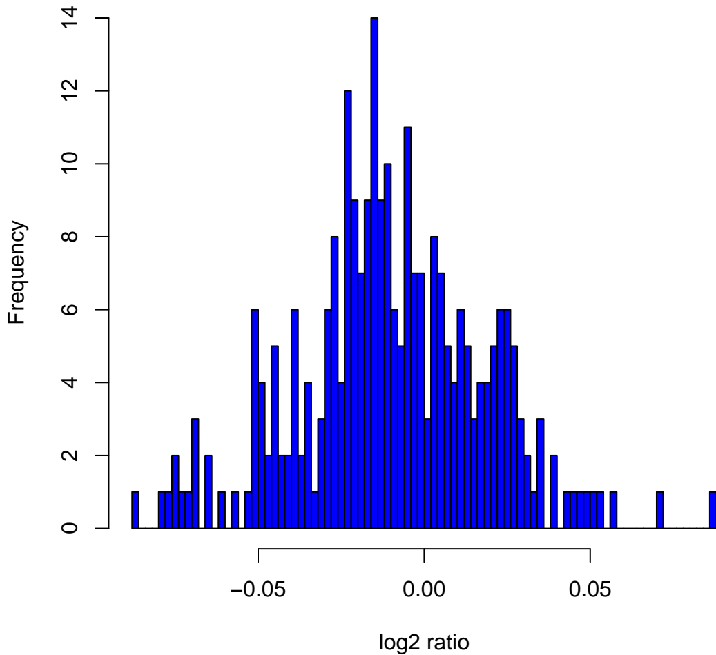
Histogram of log 2 ratios in 270 HapMap samples at clone Chr1tp-34C6
