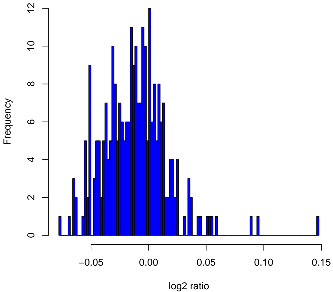
Histogram of log 2 ratios in 270 HapMap samples at clone Chr1tp-35B5
