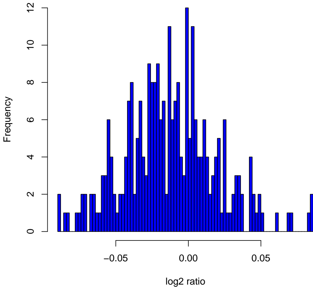
Histogram of log2ratios in 270 HapMap samples at clone Chr1tp-35D4
