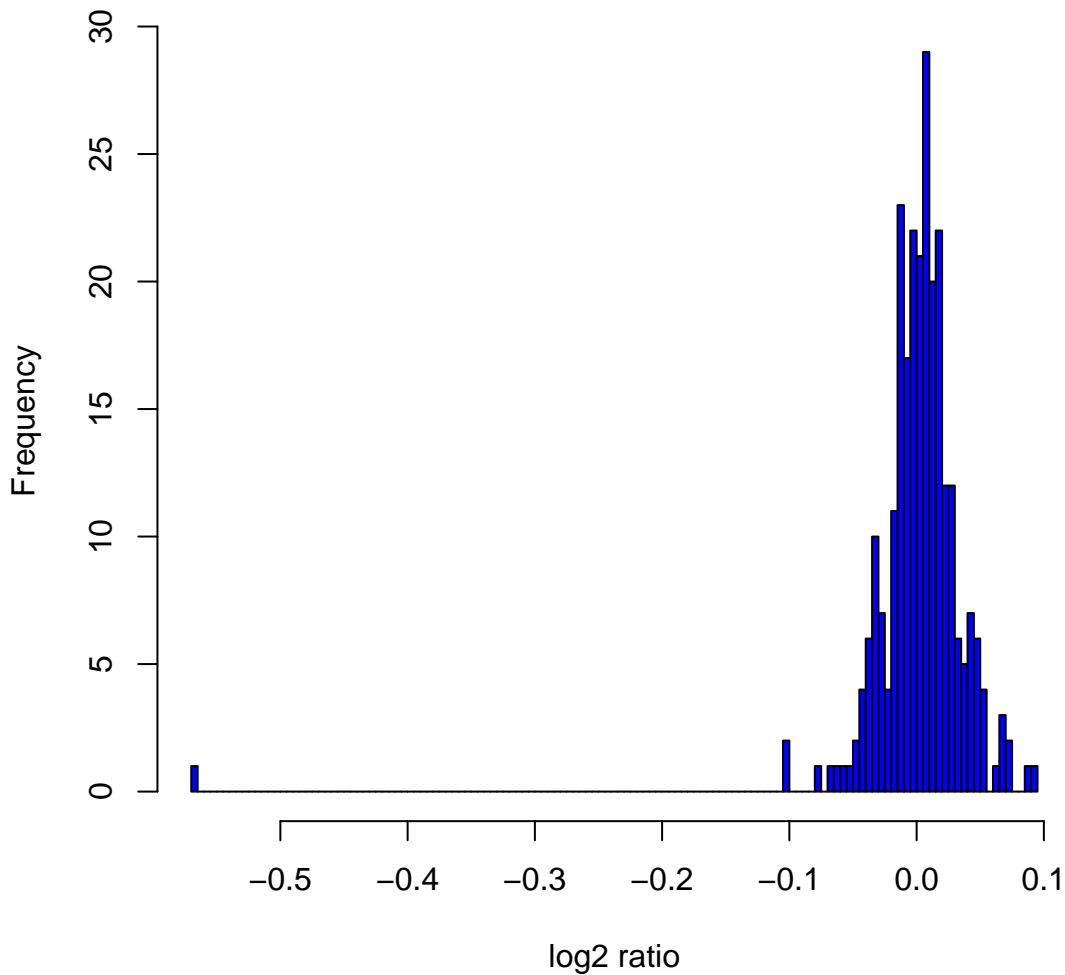
Histogram of log2ratios in 270 HapMap samples at clone Chr1tp-35E12
