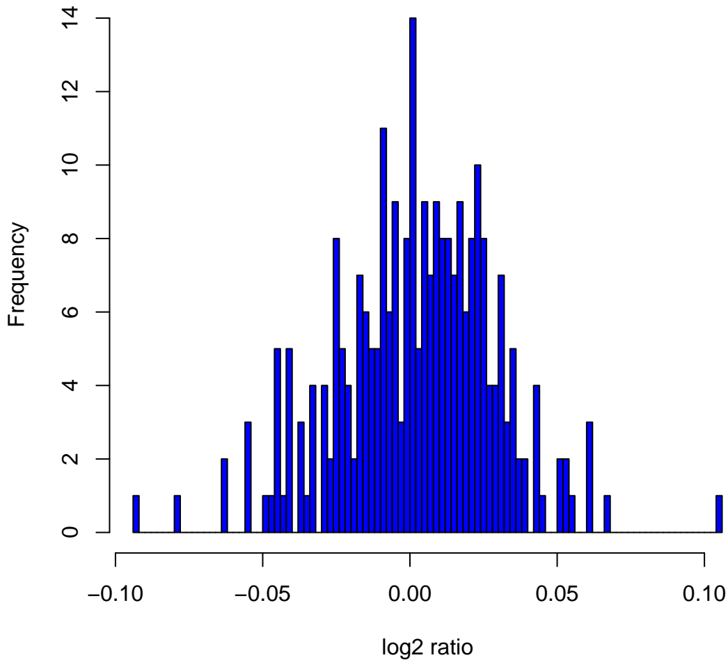
Histogram of log2ratios in 270 HapMap samples at clone Chr1tp-38B2
