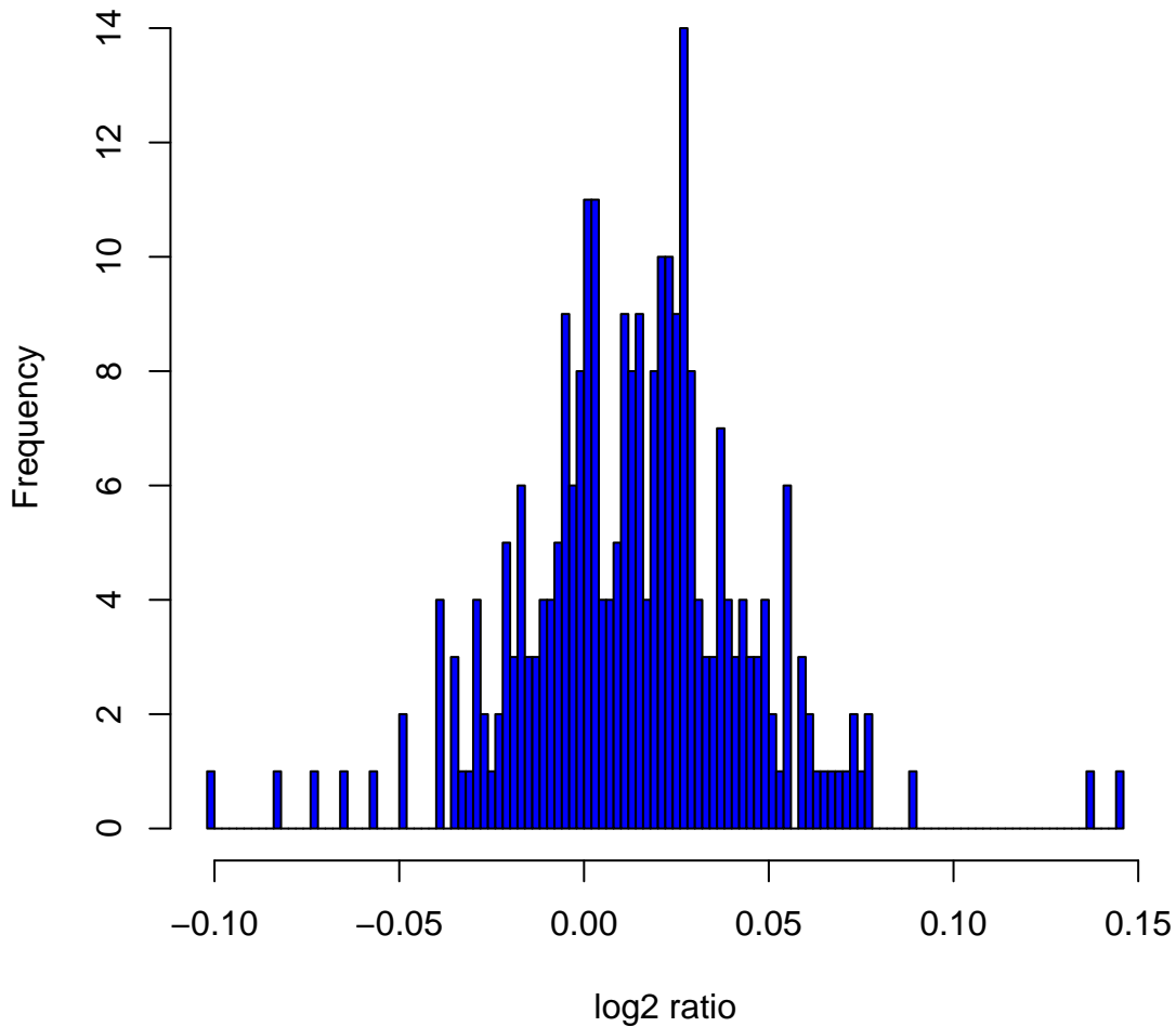
Histogram of \log_2 ratios in 270 HapMap samples at clone Chr1tp-38C10
