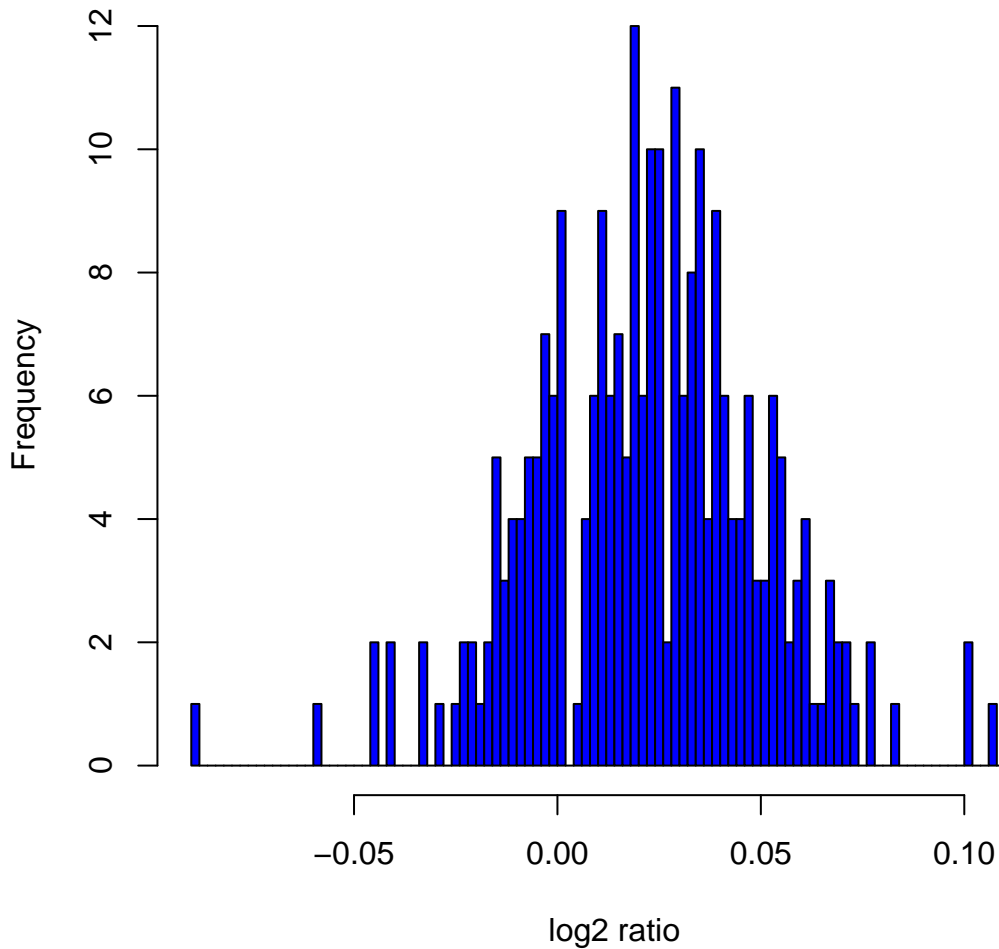
Histogram of log 2 ratios in 270 HapMap samples at clone Chr1tp-38D7
