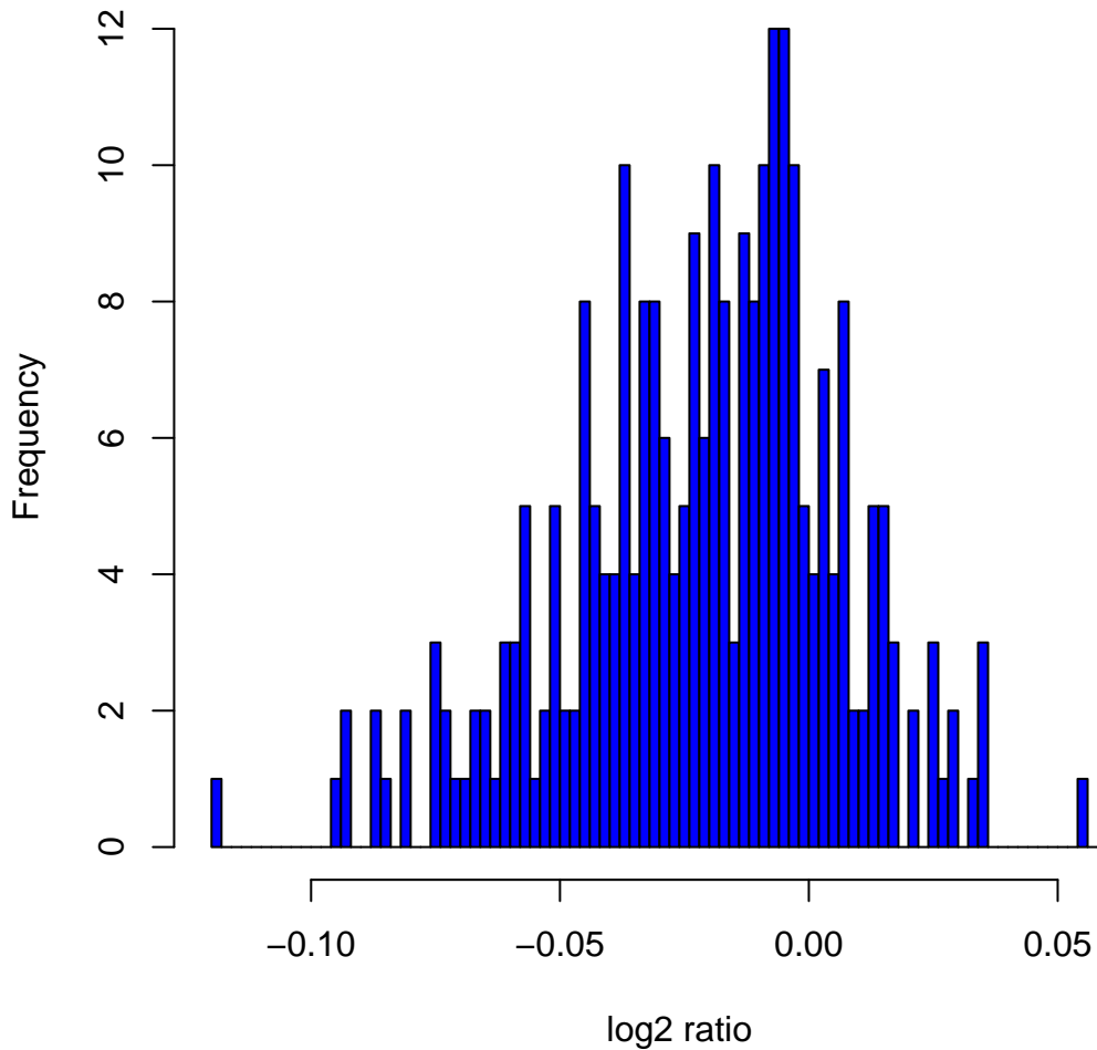
Histogram of log 2 ratios in 270 HapMap samples at clone Chr1tp-3A7
