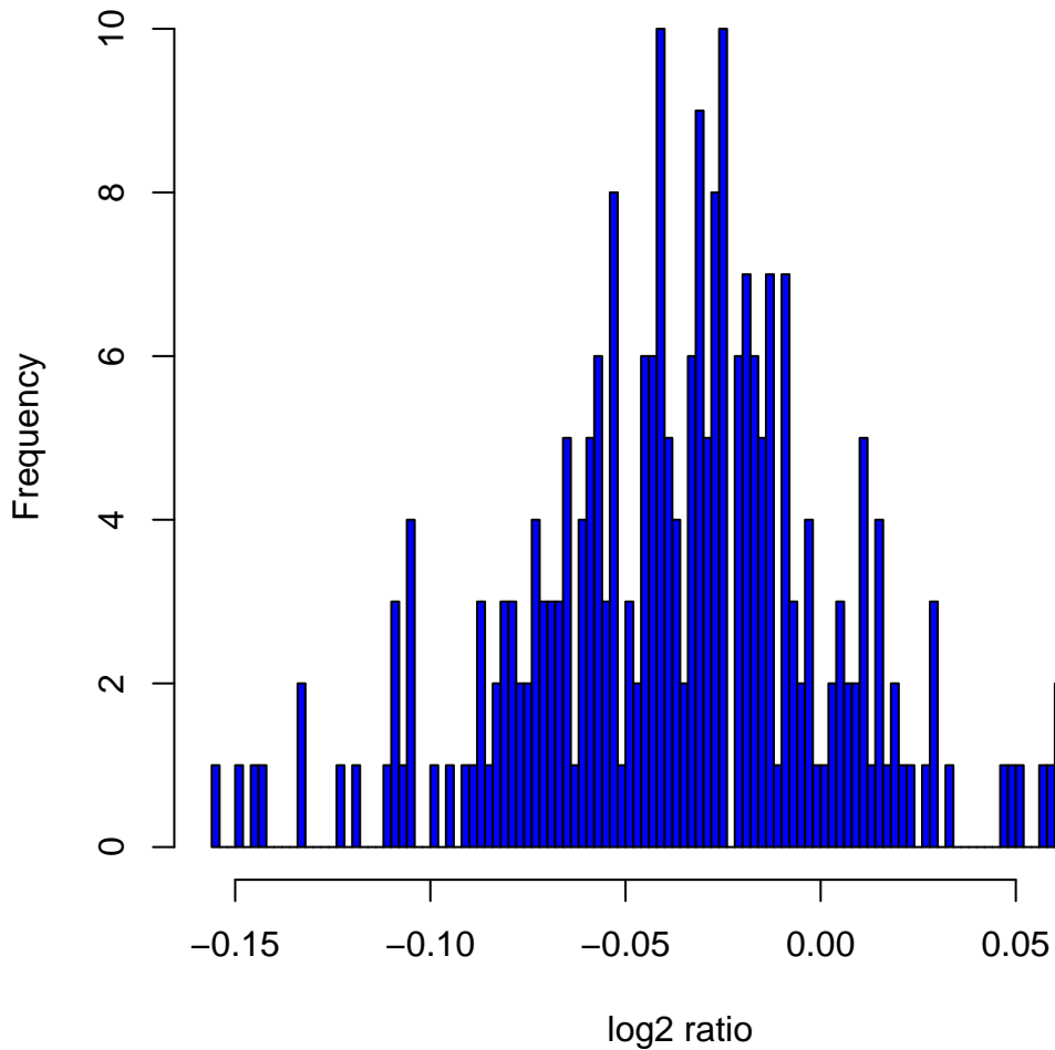
Histogram of log 2 ratios in 270 HapMap samples at clone Chr1tp-3B1
