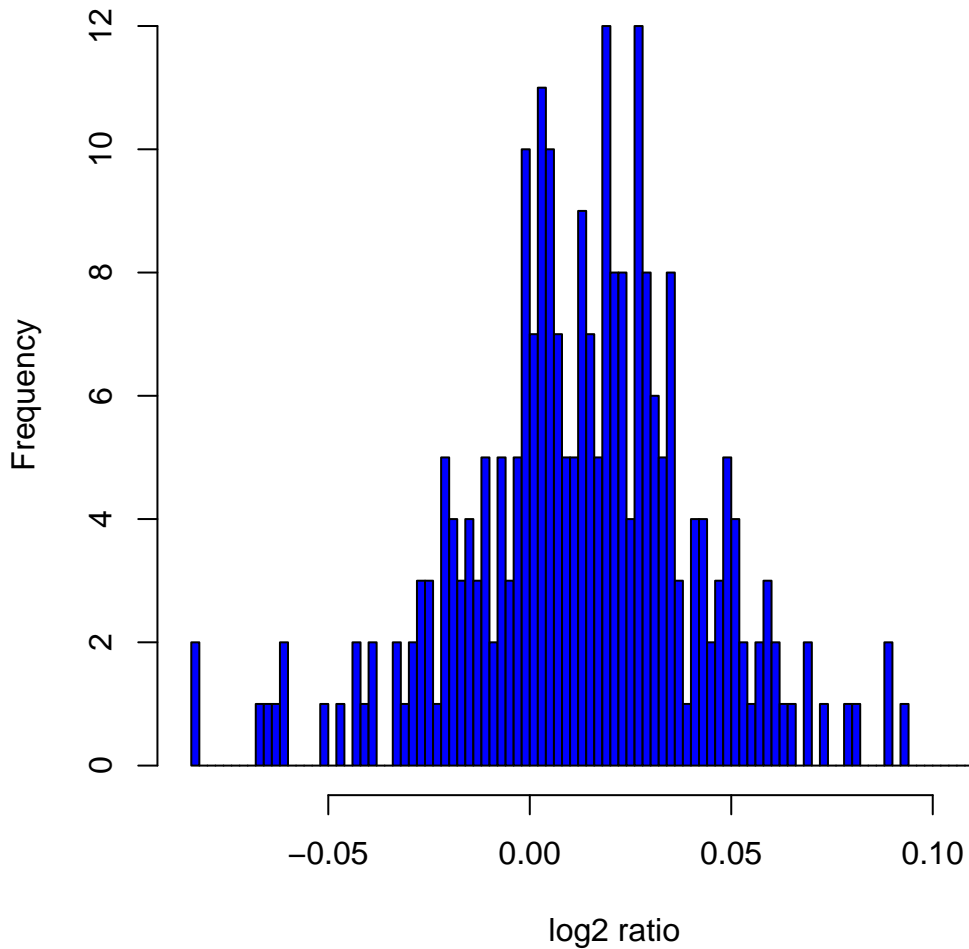
Histogram of log 2 ratios in 270 HapMap samples at clone Chr1tp-3D2
