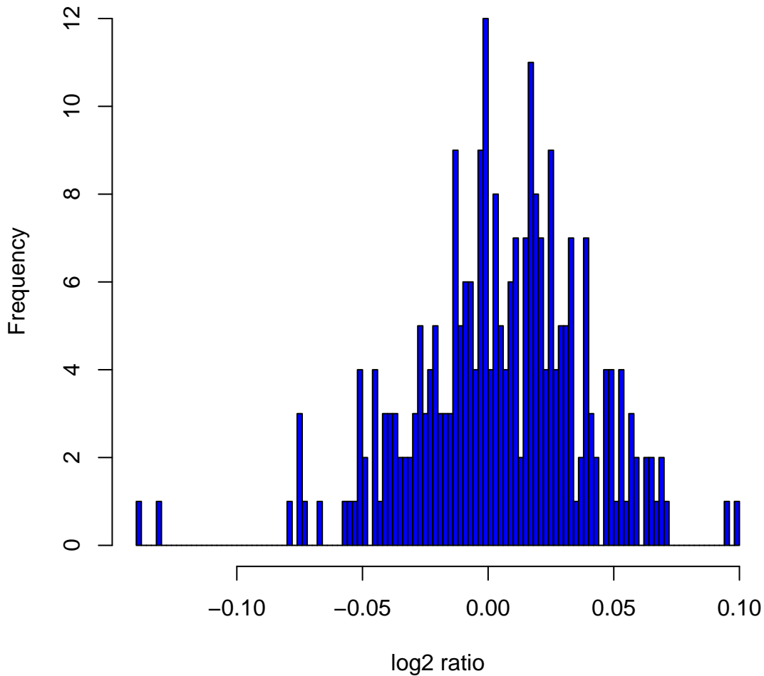
Histogram of log 2 ratios in 270 HapMap samples at clone Chr1tp-3D4
