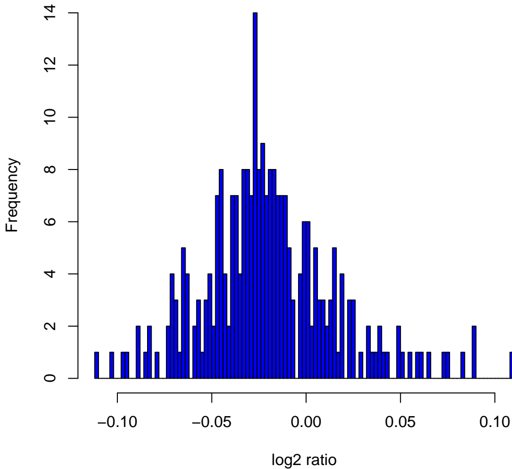
Histogram of log 2 ratios in 270 HapMap samples at clone Chr1tp-3E5
